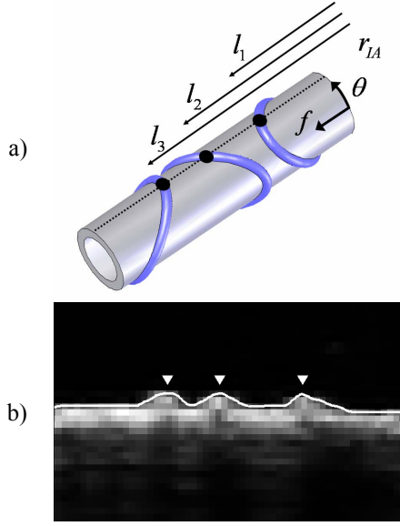
Fig. 3 - Instrument marker. a) diagram showing marker structure and measurement of l , b) 2D ultrasound image slice showing marker cross section, surface contour, and ridge locations.
