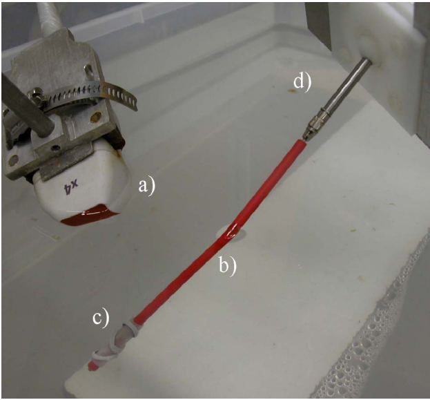
Fig. 4 - Experimental system. a) ultrasound scan head, b) instrument, c) instrument marker, d) spherical bearing. The PHANToM robot arm is not shown.
